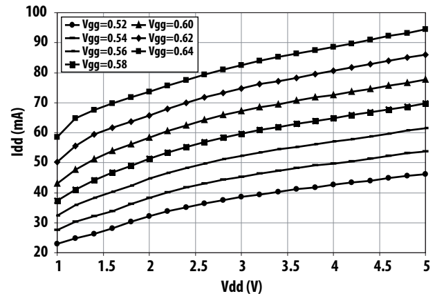
Figure 16. I-V curve
